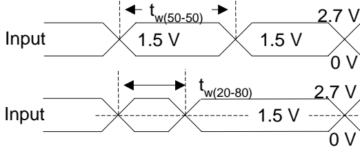
Figure 7. Voltage Waveforms—Pulse Duration
