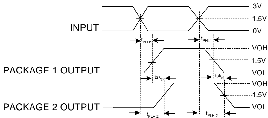
Figure 12. Output Skew— tsk_{(o)}
