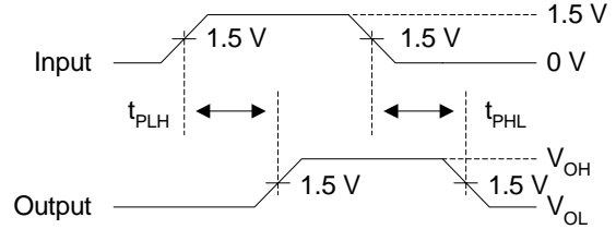
Figure 9. Voltage Waveforms—Propagation Delay Times [16]
