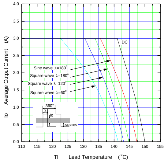
Current Derating ( I_O - T_I )
