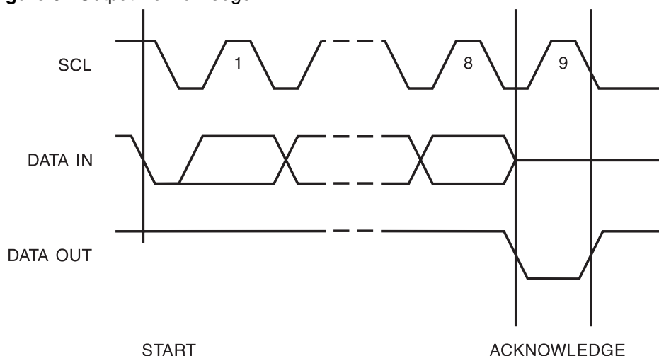
Figure 6. Output Acknowledge
