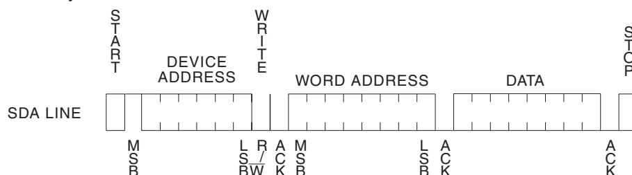
Figure 8. Byte Write
