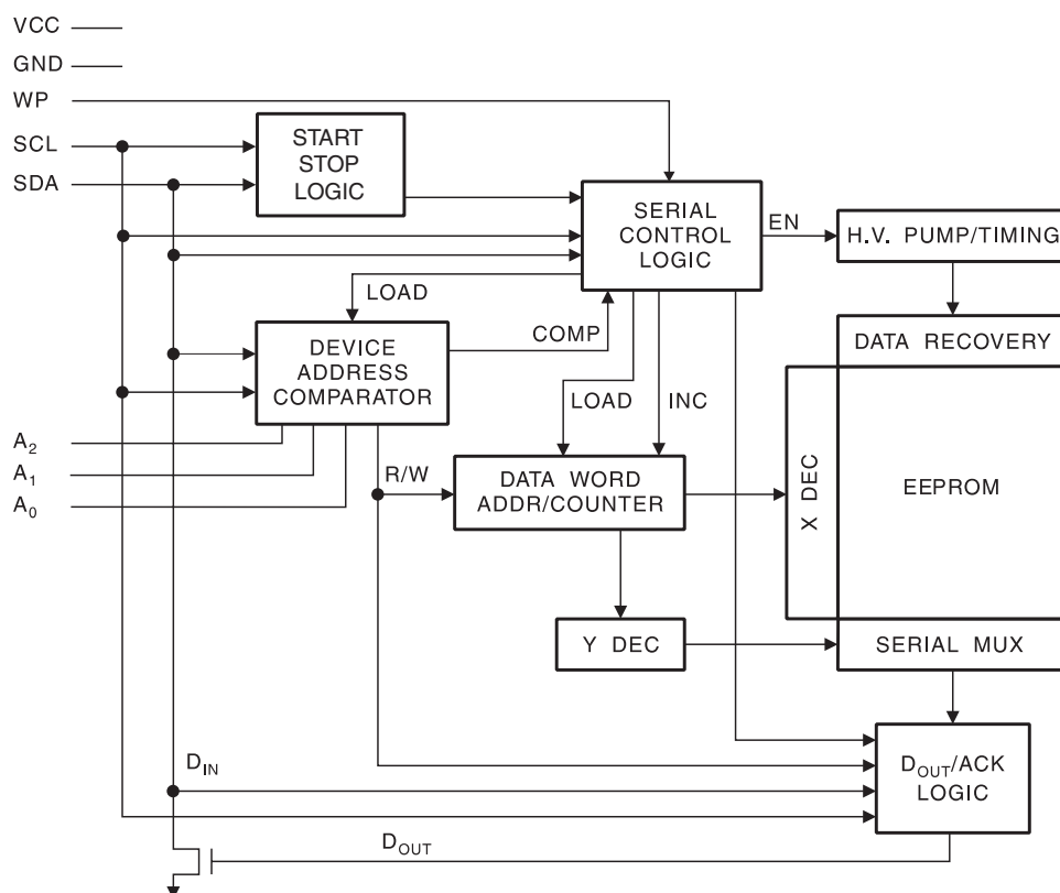
Figure 1. Block Diagram
