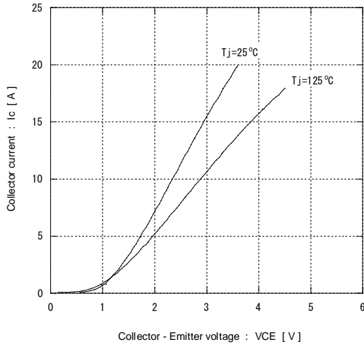
[ Brake ] Collector current vs. Collector-Emmitter voltage V_{GE} = 15\text{V}(\text{typ.}) / \text{chip}
