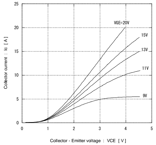
[ Brake ] Collector current vs. Collector-Emmitter voltage T_J = 125^\circ\text{C}(\text{typ.}) / \text{chip}
