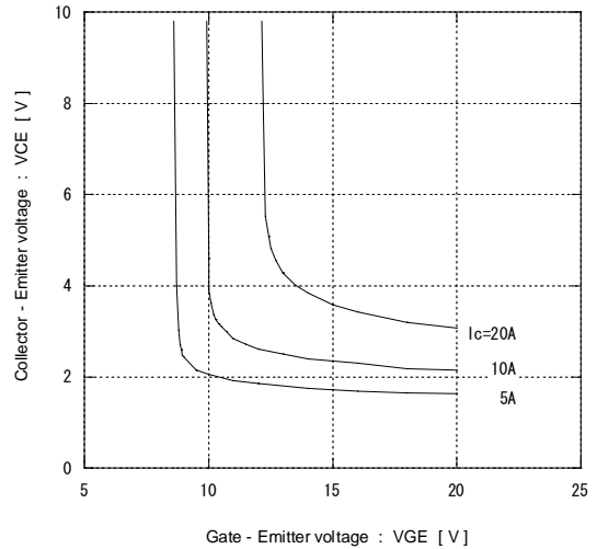
[ Brake ] Collector-Emmitter voltage vs. Gate-Emmitter voltage T_J = 25^\circ\text{C}(\text{typ.}) / \text{chip}
