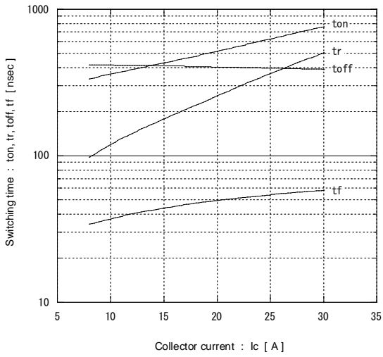
[ Inverter ] Switching time vs. Collector current (typ.) Vcc=300V, VGE=±15V, Rg=270Ω, Tj= 25°C
