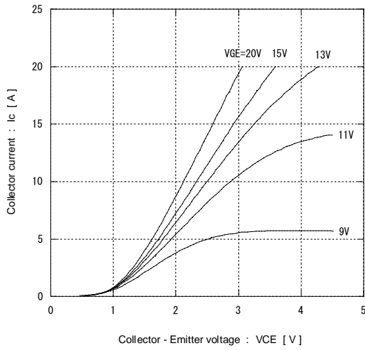
[ Brake ] Collector current vs. Collector-Emmitter voltage T_J = 25^\circ\text{C}(\text{typ.}) / \text{chip}
