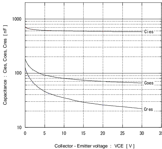
[ Brake ] Capacitance vs. Collector-Emmitter voltage (typ.) V_{GE} = 0\text{V}, f = 1\text{MHz}, T_J = 25^\circ\text{C}
