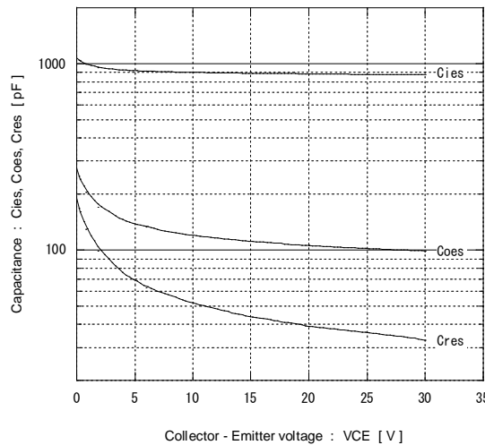
[ Inverter ] Capacitance vs. Collector-Emitter voltage (typ.) VGE = 0V, f = 1MHz, T j = 25°C
