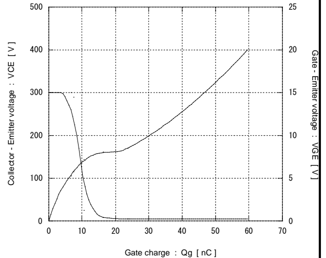
[ Inverter ] Dynamic Gate charge (typ.) Vcc = 300V, Ic = 8A, T j = 25°C
