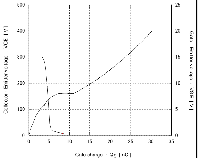
[ Brake ] Dynamic Gate charge (typ.) V_{CC} = 300\text{V}, I_C = 4\text{A}, T_J = 25^\circ\text{C}
