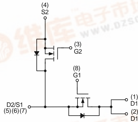
N-Channel MOSFET
