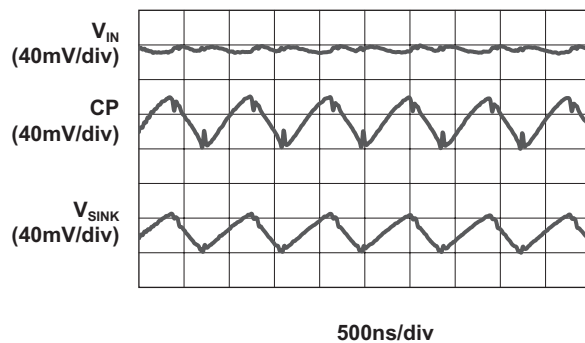
Load Characteristics ( V_{IN} = 4.0V ; 1.5X Mode; 20mA Load)
