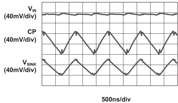
Load Characteristics ( V_{IN} = 2.9V ; 2X Mode; 15mA Load)
