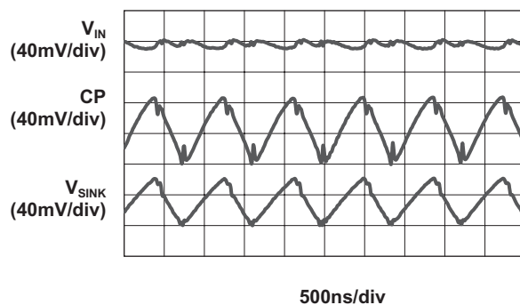
Load Characteristics ( V_{IN} = 4.3V ; 1.5X Mode; 30mA Load)
