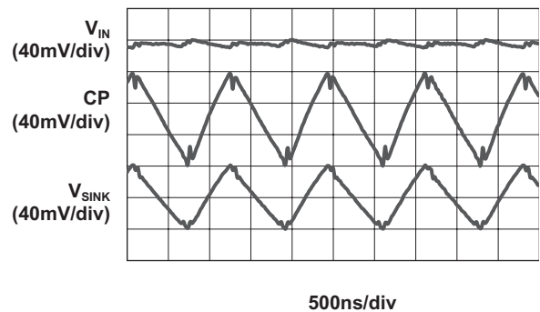
Load Characteristics ( V_{IN} = 3.1V ; 2X Mode; 20mA Load)
