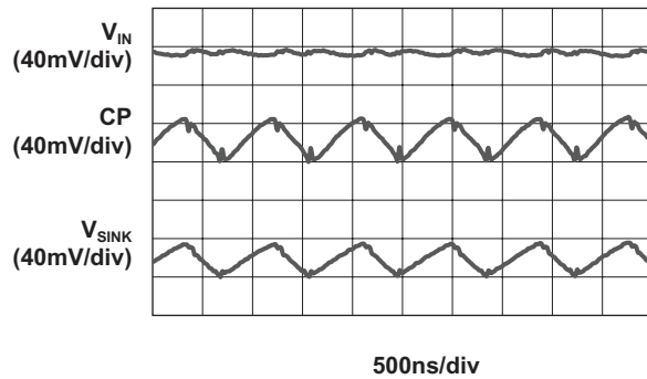
Load Characteristics ( V_{IN} = 3.8V ; 1.5X Mode; 15mA Load)
