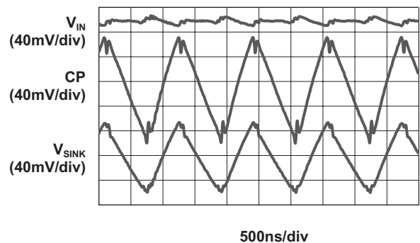
Load Characteristics ( V_{IN} = 3.6V ; 2X Mode; 30mA Load)
