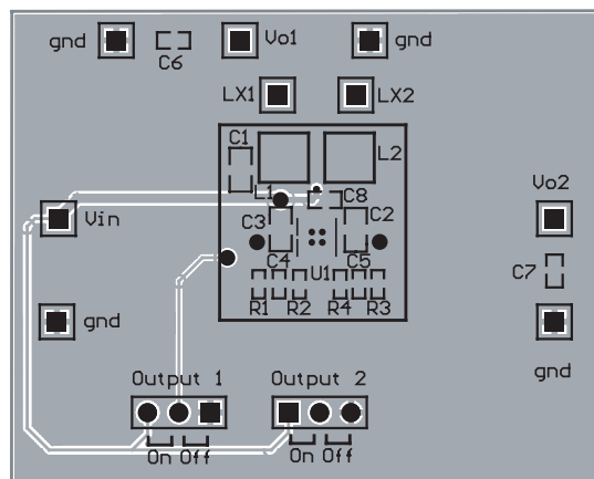
Figure 4: AAT2511 Evaluation Board Bottom Side.
