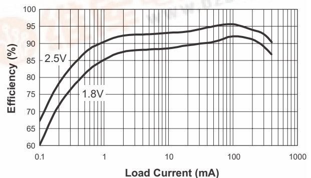
AAT2511 Efficiency ( V_{IN} = 3.3V )
