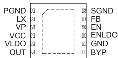
TDFN/STDFN33-12 (TopView)
