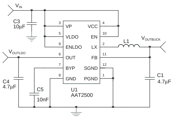
Figure 1: AAT2500 Fixed Output.
