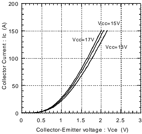
Collector current vs. Collector-Emmitter voltage Tj=125°C(Chip)
