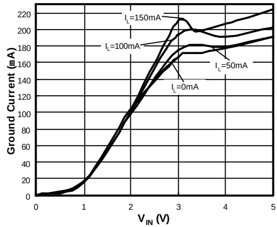
Ground Current vs V_{IN} @ 125^\circ\text{C}
