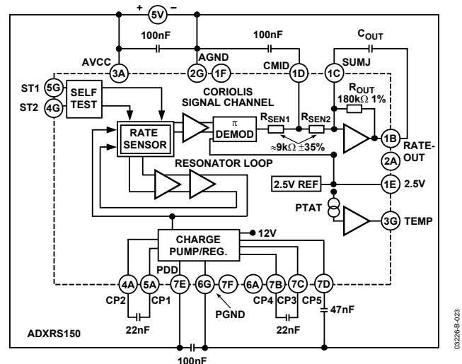
Figure 23. Block Diagram with External Components
