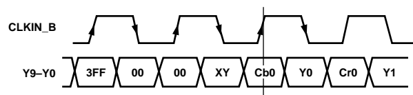
Figure 54. Input Sequence in PS Bit Interleaved Mode (EAV/SAV)
