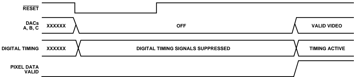
Figure 63. RESET Timing Sequence
