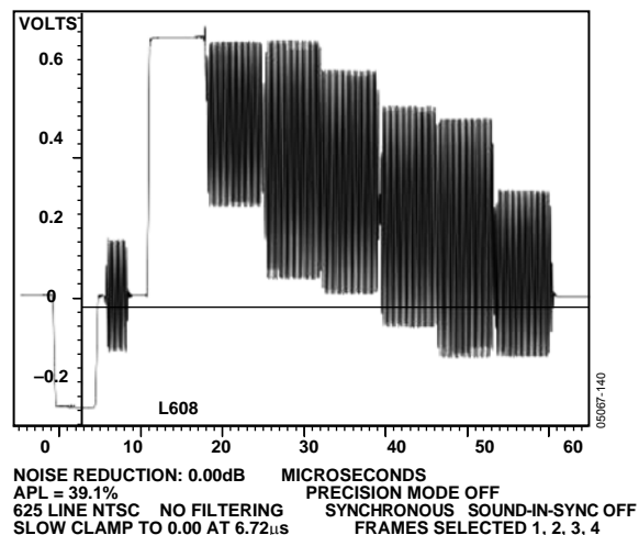
Figure 140. PAL Color Bars 75%
