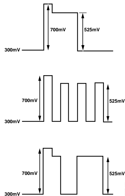
Figure 129. SD RGB Output Levels—RGB Sync Disabled
