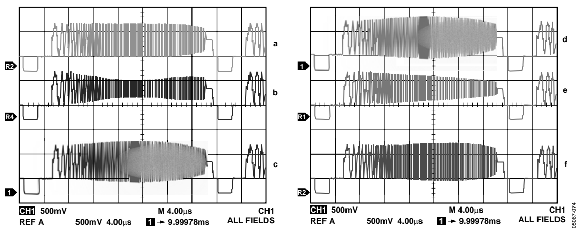
Figure 74. HD Sharpness Filter Control with Different Gain Settings for HS Sharpness Filter Gain Values
