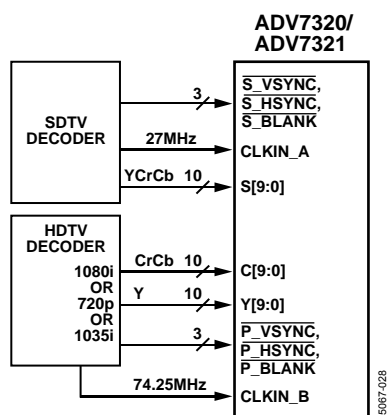
Figure 52. Simultaneous HD and SD Input
