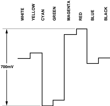
Figure 134. Pr Levels—PAL
