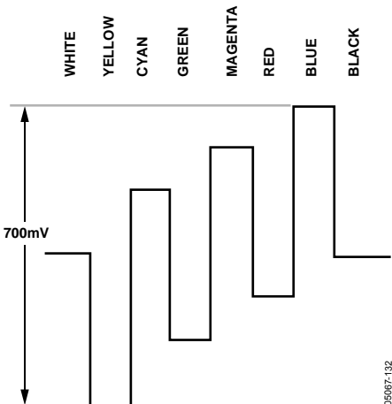
Figure 132. Pb Levels—PAL
