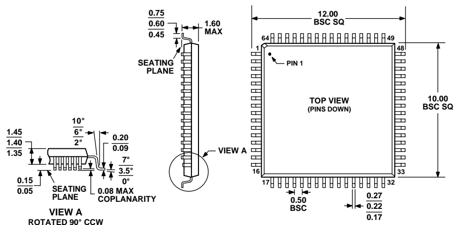
Figure 149. 64-Lead Low Profile Quad Flat Package [LQFP] (ST-64-2)
