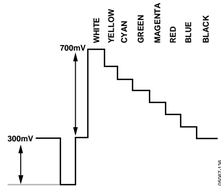
Figure 135. Y Levels—NTSC
