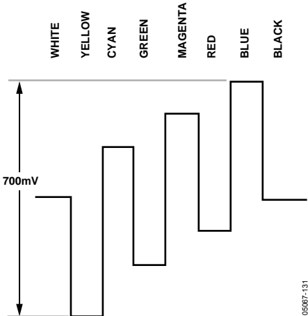
Figure 131. Pb Levels—NTSC
