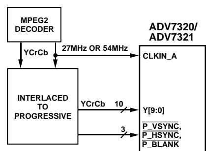
Figure 57. 10-Bit PS at 27 MHz or 54 MHz
