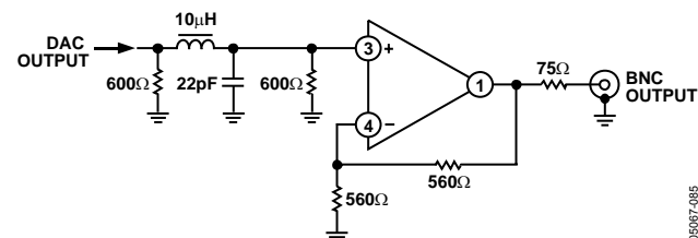
Figure 85. Example of Output Filter for SD, 16x Oversampling
