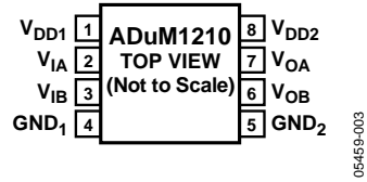
Figure 3. Pin Configuration
