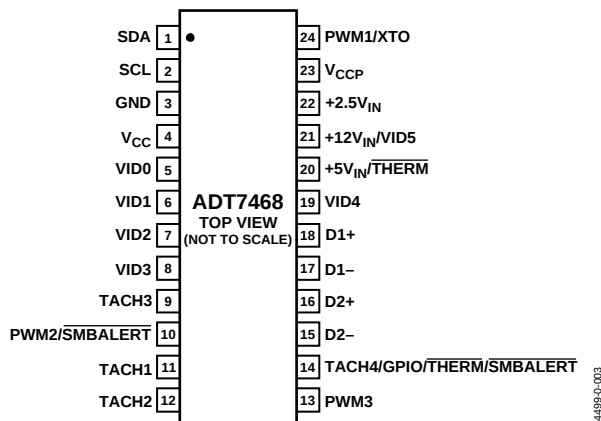
Figure 3. Pin Configuration
