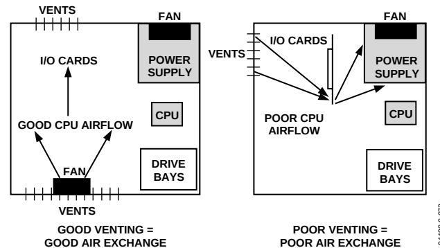
Figure 50. Chassis Airflow Issues
