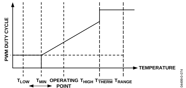
Figure 52. Dynamic T_{MIN} Control Loop
