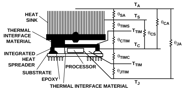
Figure 51. Thermal Model
