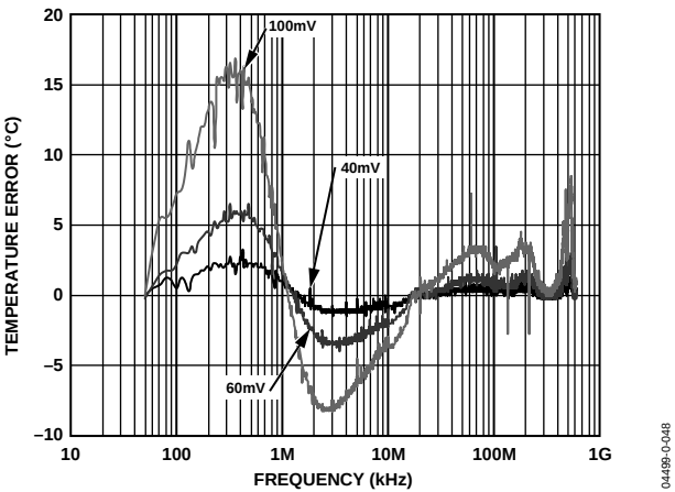
Figure 7. Remote Temperature Error vs. Common Mode Noise Frequency
