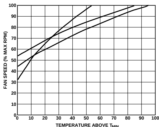
Figure 67. T_{\text{RANGE}} and % Fan Speed Slopes for VRM, Ambient, and CPU Temperature Channels
