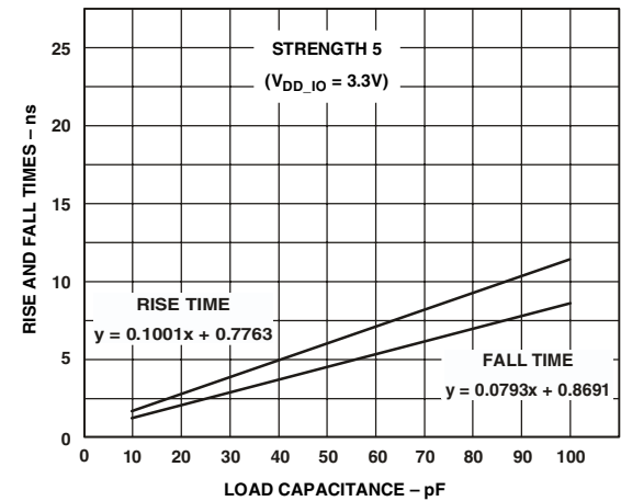
Figure 36. Typical Output Rise and Fall Time (10%–90%, V_{DD\_IO} = 3.3\text{ V} ) vs. Load Capacitance at Strength 5
