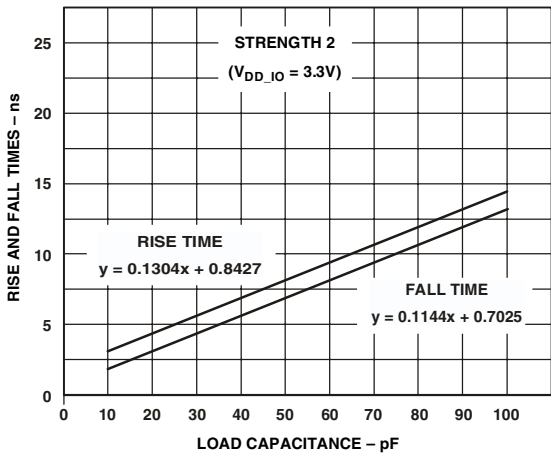
Figure 33. Typical Output Rise and Fall Time (10%–90%, V_{DD\_IO} = 3.3\text{ V} ) vs. Load Capacitance at Strength 2
