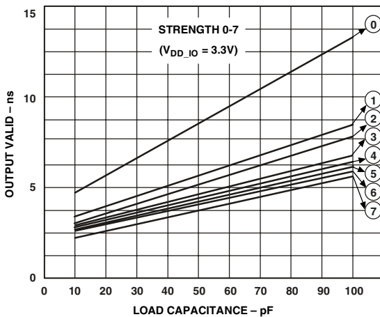
Figure 39. Typical Output Valid (V DD_IO = 3.3 V) vs. Load Capacitance at Max Case Temperature and Strength 0–7 1
