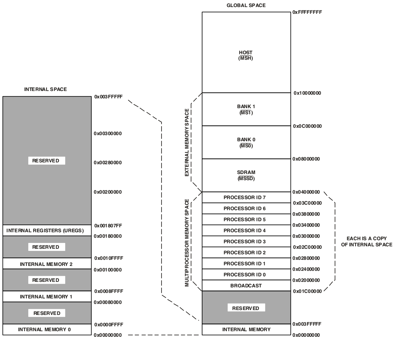
Figure 3. Memory Map
