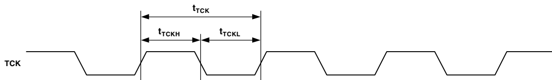
Figure 11. Reference Clocks—Test Clock (TCK) Cycle Time
