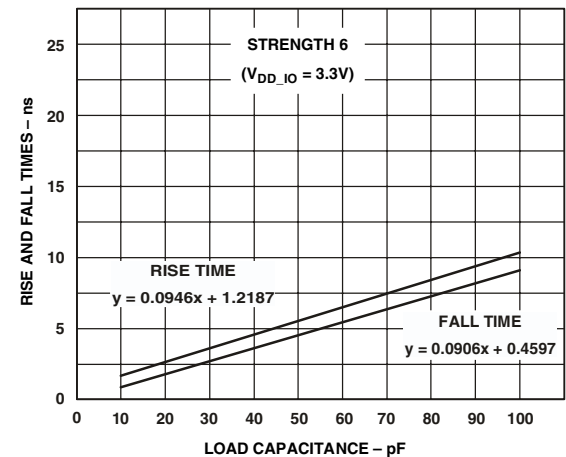
Figure 37. Typical Output Rise and Fall Time (10%–90%, V_{DD\_IO} = 3.3\text{ V} ) vs. Load Capacitance at Strength 6
