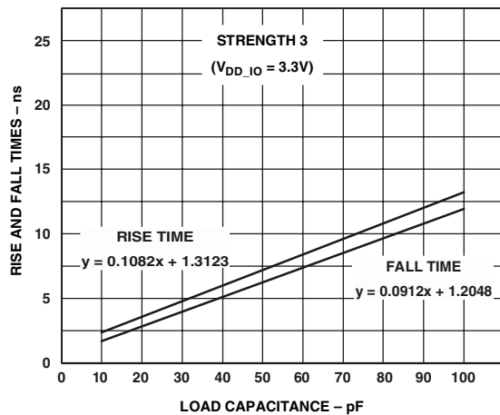
Figure 34. Typical Output Rise and Fall Time (10%–90%, V_{DD\_IO} = 3.3\text{ V} ) vs. Load Capacitance at Strength 3
