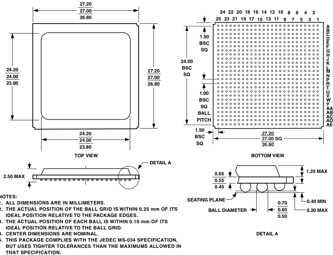
Figure 43. 625-Ball PBGA (B-625)
