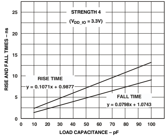
Figure 35. Typical Output Rise and Fall Time (10%–90%, V_{DD\_IO} = 3.3\text{ V} ) vs. Load Capacitance at Strength 4
