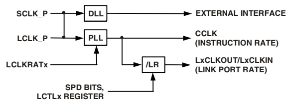
Figure 5. Clock Domains
