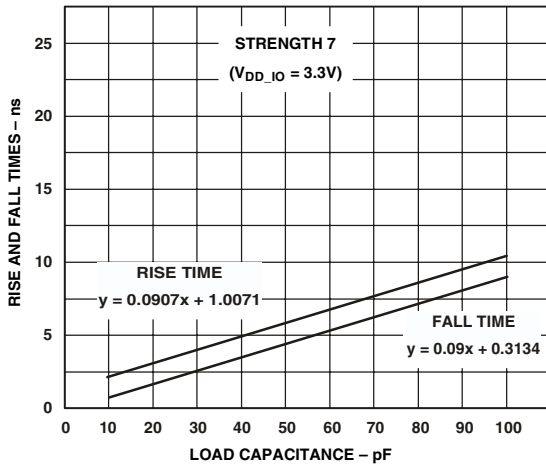
Figure 38. Typical Output Rise and Fall Time (10%–90%, V DD_IO = 3.3 V) vs. Load Capacitance at Strength 7
