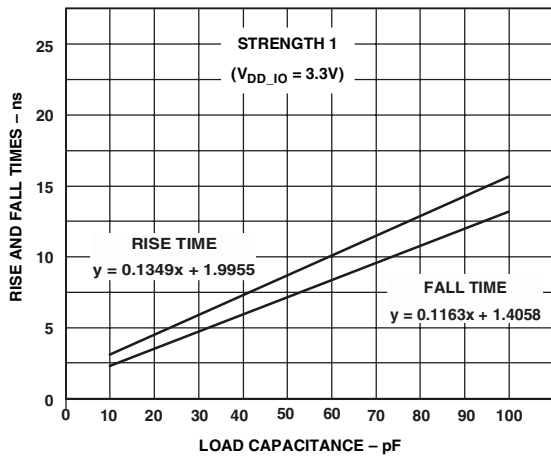
Figure 32. Typical Output Rise and Fall Time (10%–90%, V_{DD\_IO} = 3.3\text{ V} ) vs. Load Capacitance at Strength 1
