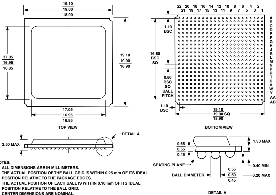
Figure 42. 484-Ball PBGA (B-484)
