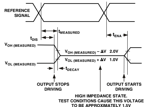
Figure 18. Output Enable/Disable
