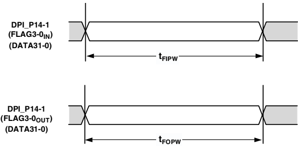
Figure 14. Flags
