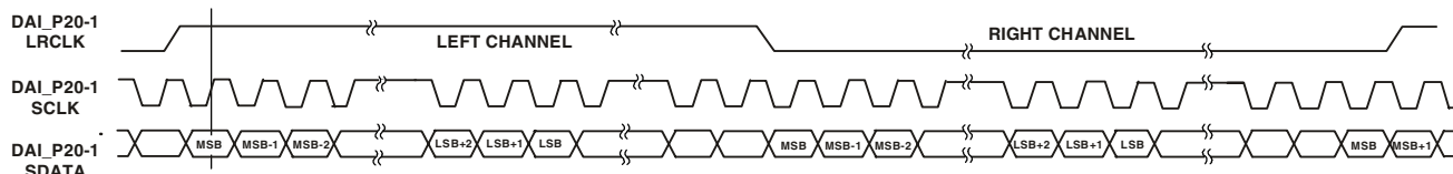
Figure 28. Left-Justified Mode
