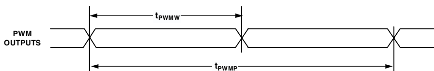
Figure 23. PWM Timing
