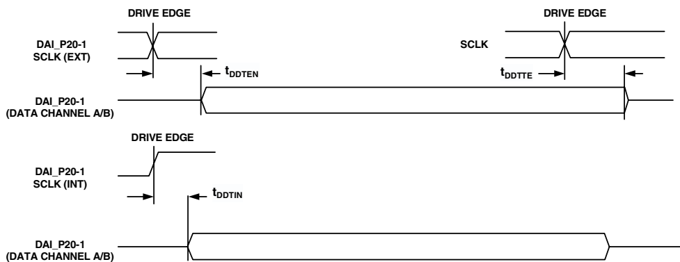
Figure 20. Serial Ports
