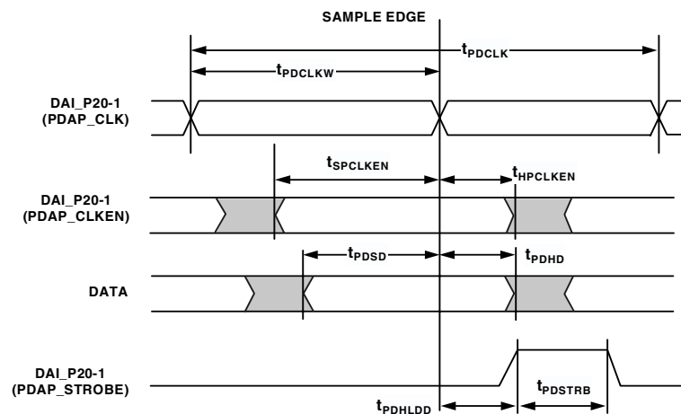
Figure 22. PDAP Timing
