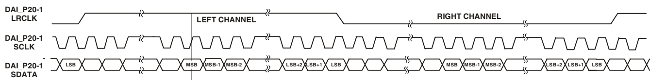
Figure 26. Right-Justified Mode
