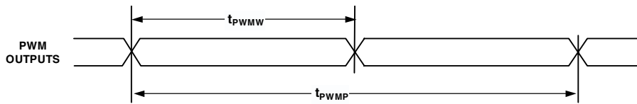
Figure 25. PWM Timing
