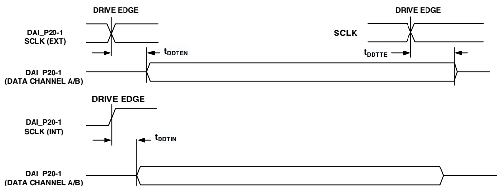
Figure 22. Serial Ports
