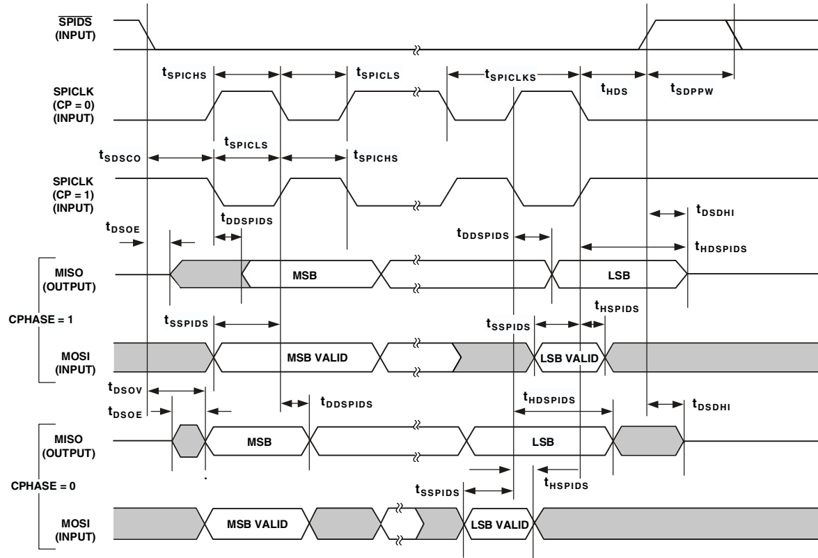
Figure 27. SPI Slave Timing
