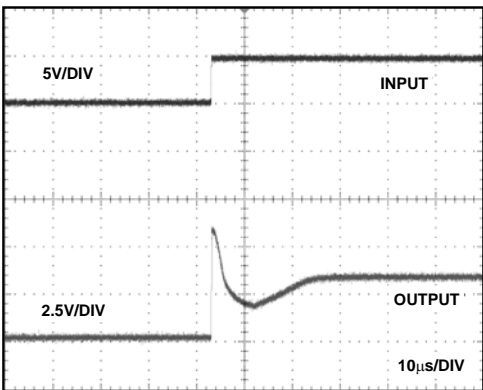
Figure 28. ADR361 Turn-On Response Time at 5 V
