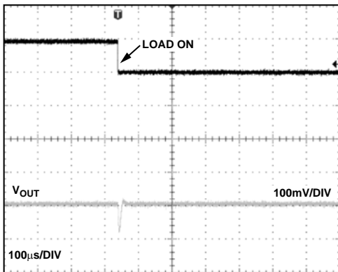
Figure 27. ADR361 Load Transient Response, 0.1 \mu F Input, Output Capacitor
