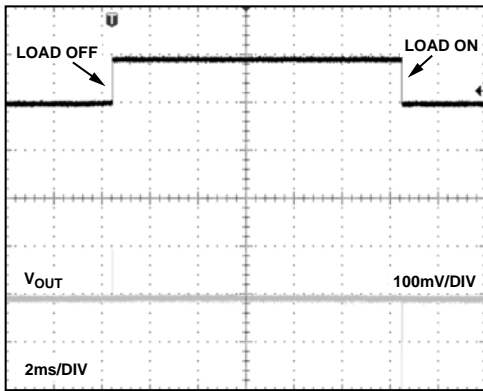
Figure 26. ADR361 Load Transient Response
