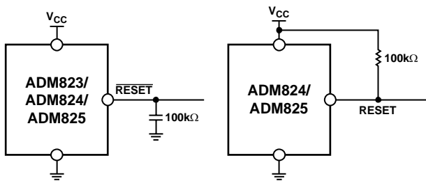
Figure 17. Ensuring Reset Valid to V_{CC} = 0\text{ V}
