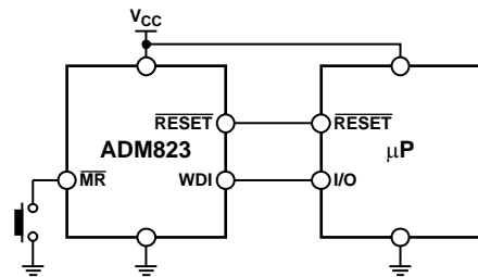
Figure 19. Typical Application Circuit
