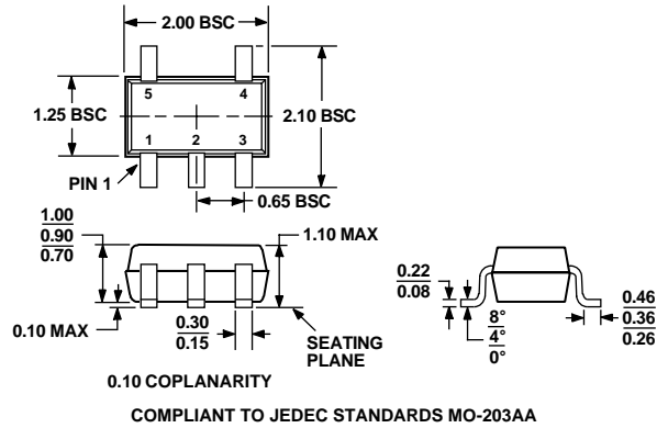
Figure 20. 5-Lead Plastic Surface-Mount Package [SC-70] (KS-5) Dimensions shown in millimeters
