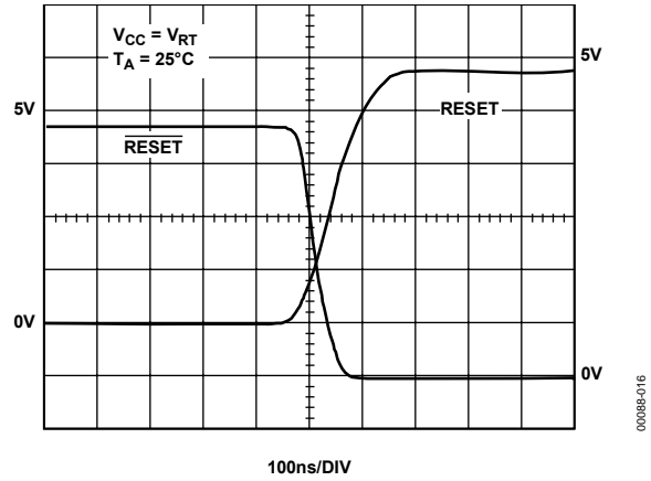
Figure 9. \overline{\text{RESET}} , \text{RESET} Assertion
