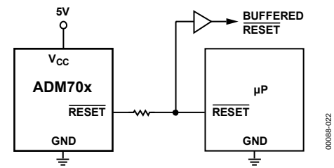
Figure 20. Bidirectional I-O RESET
