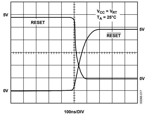
Figure 10. \overline{\text{RESET}} , \text{RESET} Deassertion
