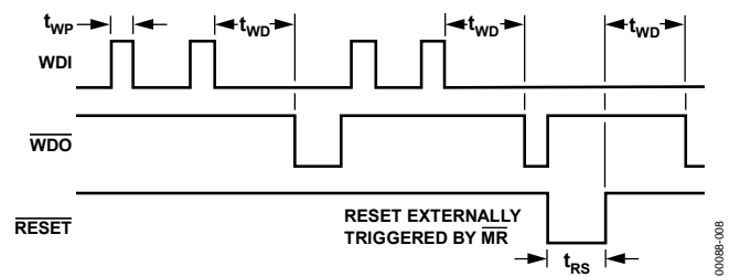
Figure 13. Watchdog Timing
