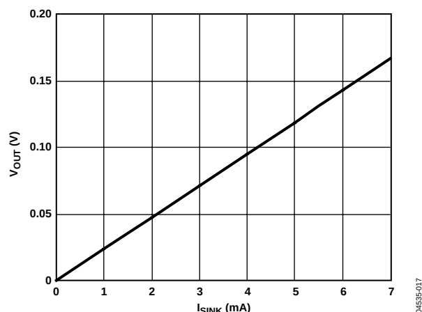
Figure 8. Output Voltage Low vs. I_{SINK}
