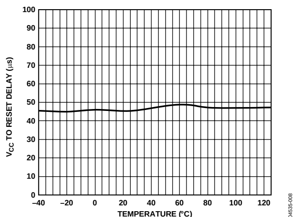
Figure 5. V_{CC} to RESET Output Delay vs. Temperature
