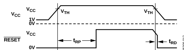
Figure 12. Reset Timing Diagram
