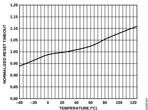
Figure 6. Normalized Reset Timeout Period vs. Temperature
