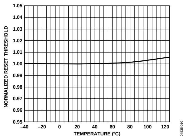
Figure 7. Normalized Reset Threshold vs. Temperature
