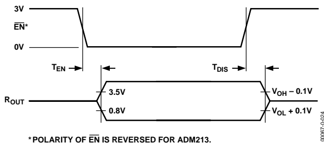
Figure 24. Enable Timing
