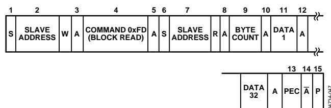
Figure 36. Block Read from EEPROM or RAM with PEC
