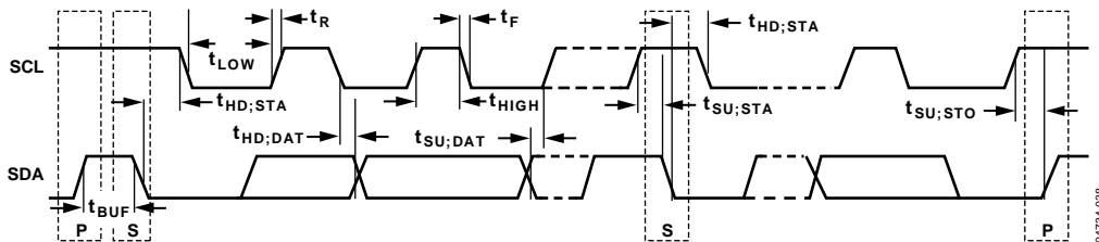
Figure 27. Serial Bus Timing Diagram
