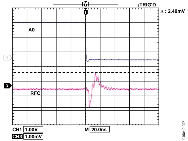
Figure 16. Video Feedthrough
