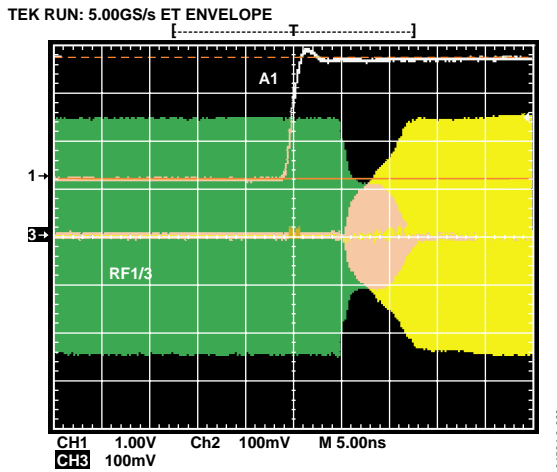
Figure 15. Switch Timing
