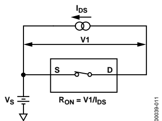
Figure 11. On Resistance
