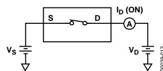
Figure 13. On Leakage
