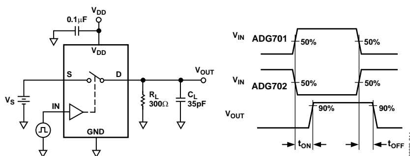
Figure 14. Switching Times
