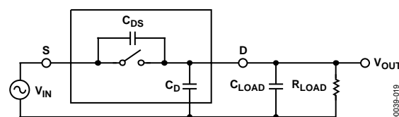
Figure 19. Off Isolation Is Affected by External Load Resistance and Capacitance
