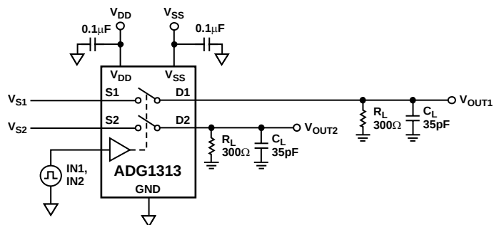
Figure 14. Test Circuit 5—Break-Before-Make Time Delay
