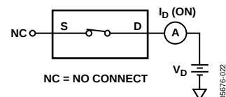
Figure 12. Test Circuit 3—On Leakage
