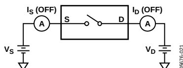
Figure 11. Test Circuit 2—Off Leakage
