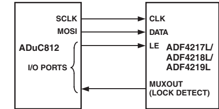
Figure 9. ADuC812 to ADF421xL Interface
