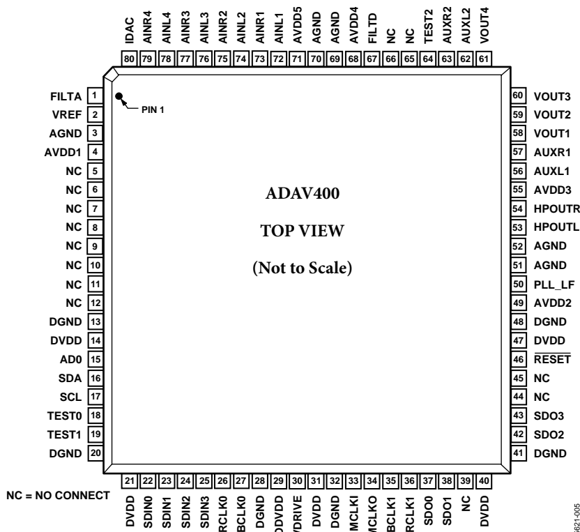
Figure 5. Pin Configuration
