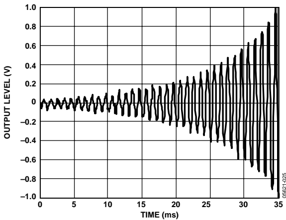
Figure 26. Slew RAM—Constant dB Update Increasing Ramp
