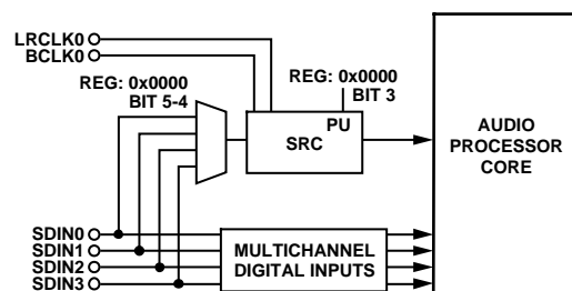
Figure 18. SRC Input Configuration
