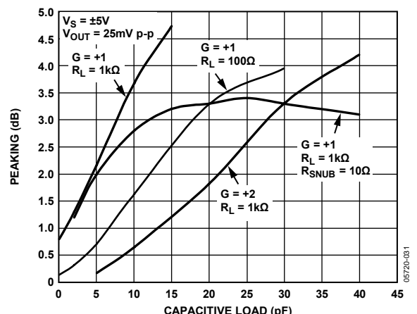
Figure 10. Small Signal Frequency Response Peaking vs. Capacitive Load for Various Gains
