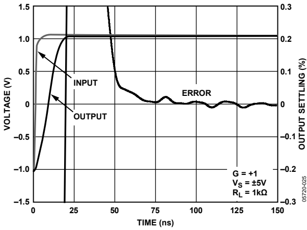
Figure 29. Settling Time
