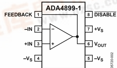
Figure 2. 8-Lead SOIC_N_EP (RD-8-1)
