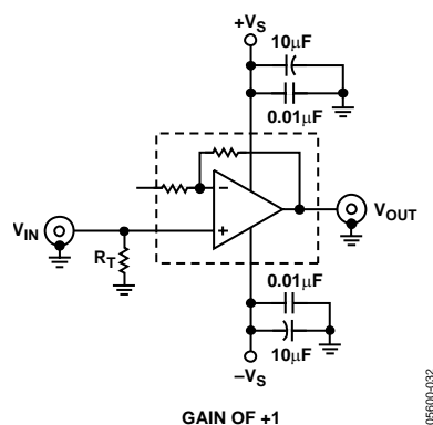
Figure 30. Unity Gain of Option 1
