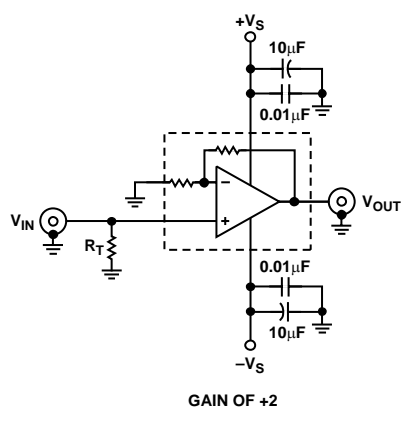
Figure 29. Noninverting Configuration ( G = +2 )
