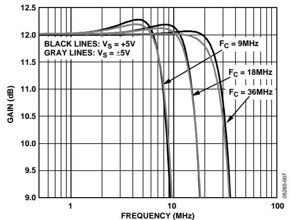
Figure 8. Frequency Response Flatness vs. Cutoff Frequency ( G = \times 4 )
