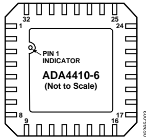
Figure 3. 32-Lead LFCSP, Top View
