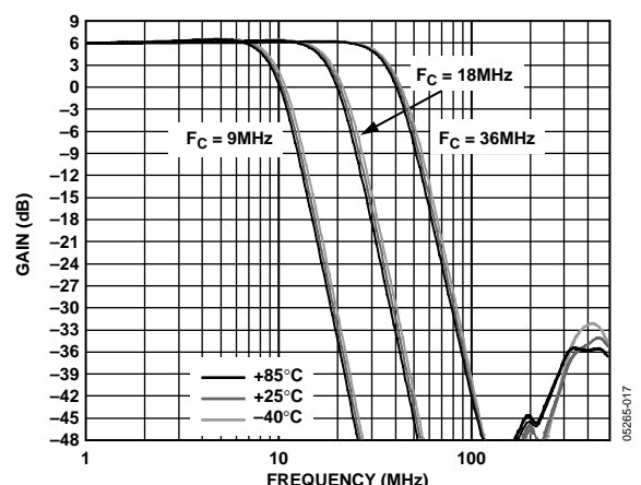
Figure 9. Frequency Response vs. Temperature and Cutoff Frequency
