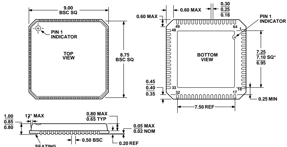
Figure 87. 64-Lead Lead Frame Chip Scale Package (LFCSP) [CP-64]
