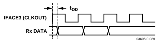
Figure 86. Rx Data Timing Diagram
