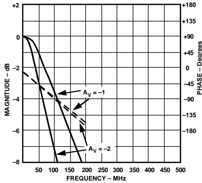
Figure 5. Inverting Frequency Response
