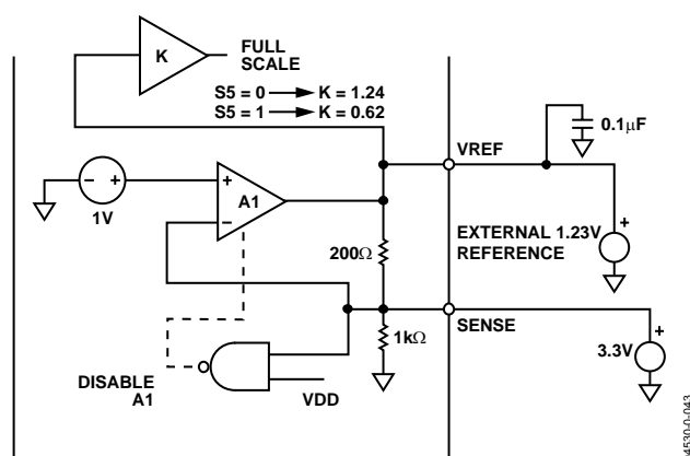
Figure 43. Using an External Reference
