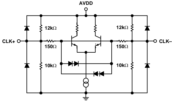
Figure 4. Clock Inputs
