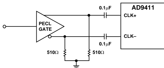
Figure 39. Driving Clock Inputs with LVEL16
