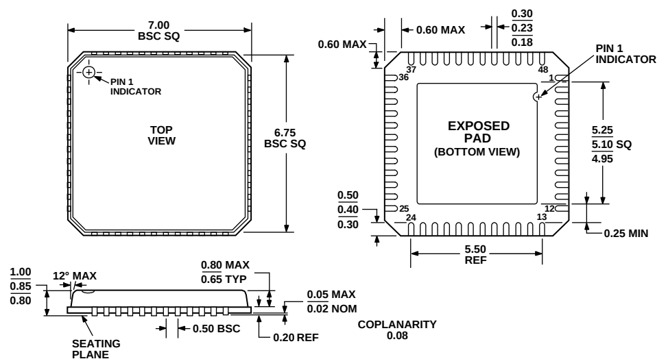
Figure 55. 48-Lead Frame Chip Scale Package [LFCS] (CP-48-1)
