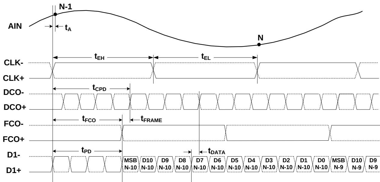
Figure 2. Timing Diagram
