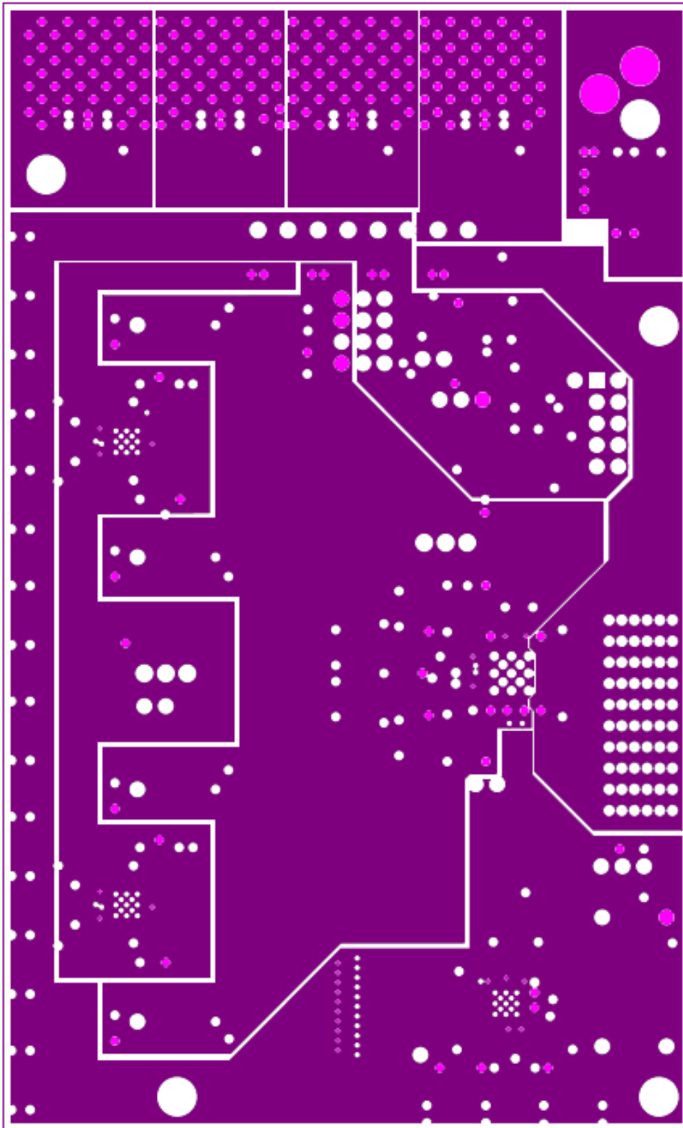
Figure 53. Evaluation Board Layout, Power Plane
