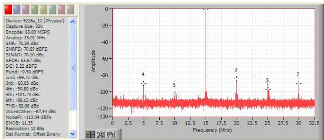
Figure 9. Single-Tone 32k FFT with f_{IN} = 15\text{ MHz} , f_{SAMPLE} = 65\text{ MSPS}
