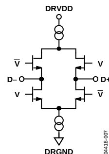
Figure 6. Equivalent Digital Output Circuit
