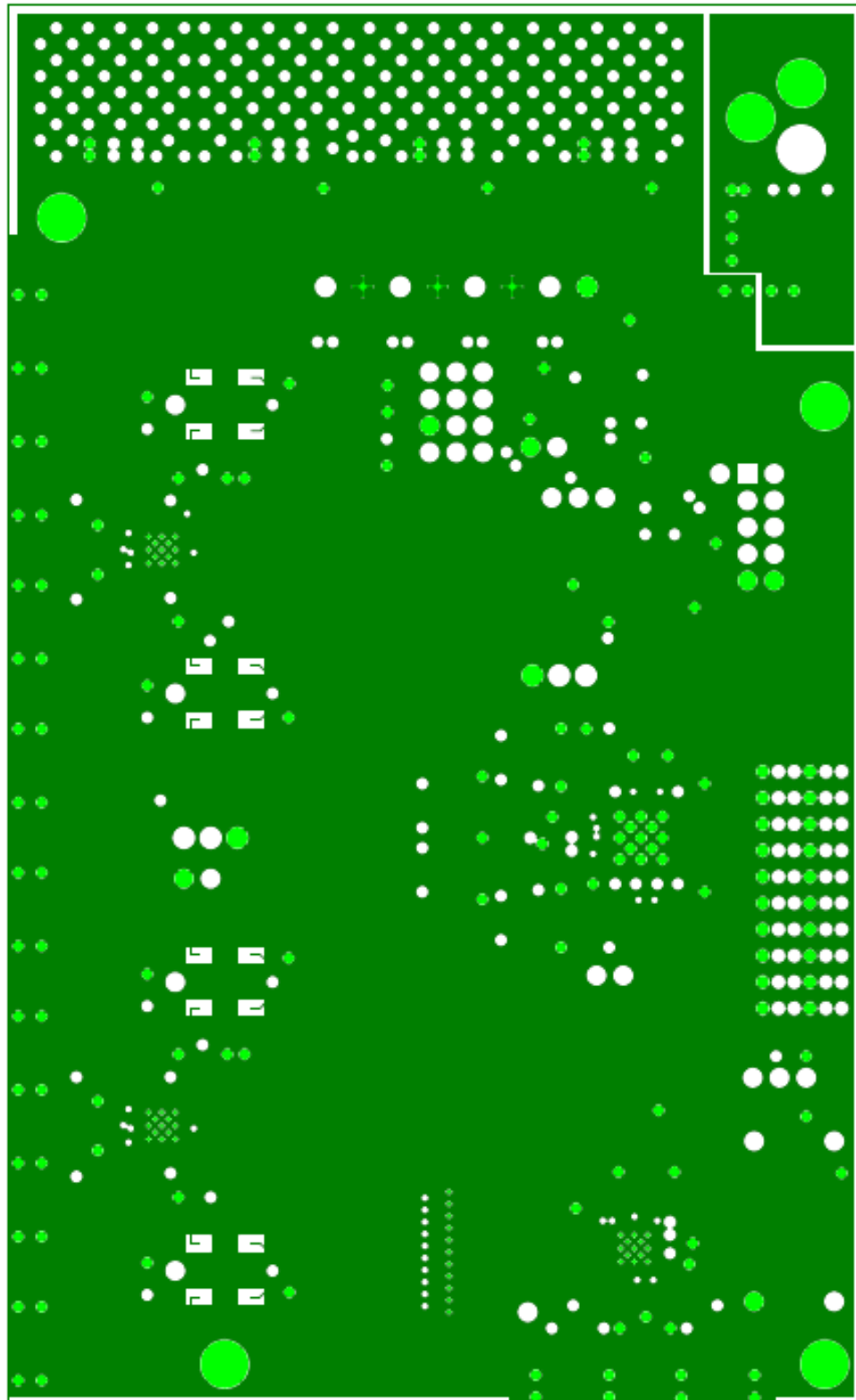
Figure 52. Evaluation Board Layout, Ground Plane
