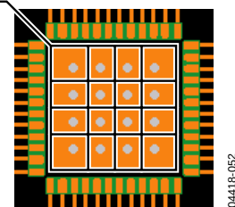
Figure 47. Typical PCB Layout
