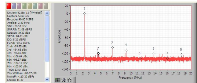
Figure 8. Single-Tone 32k FFT with f_{IN} = 2.3\text{ MHz} , f_{SAMPLE} = 40\text{ MSPS}
