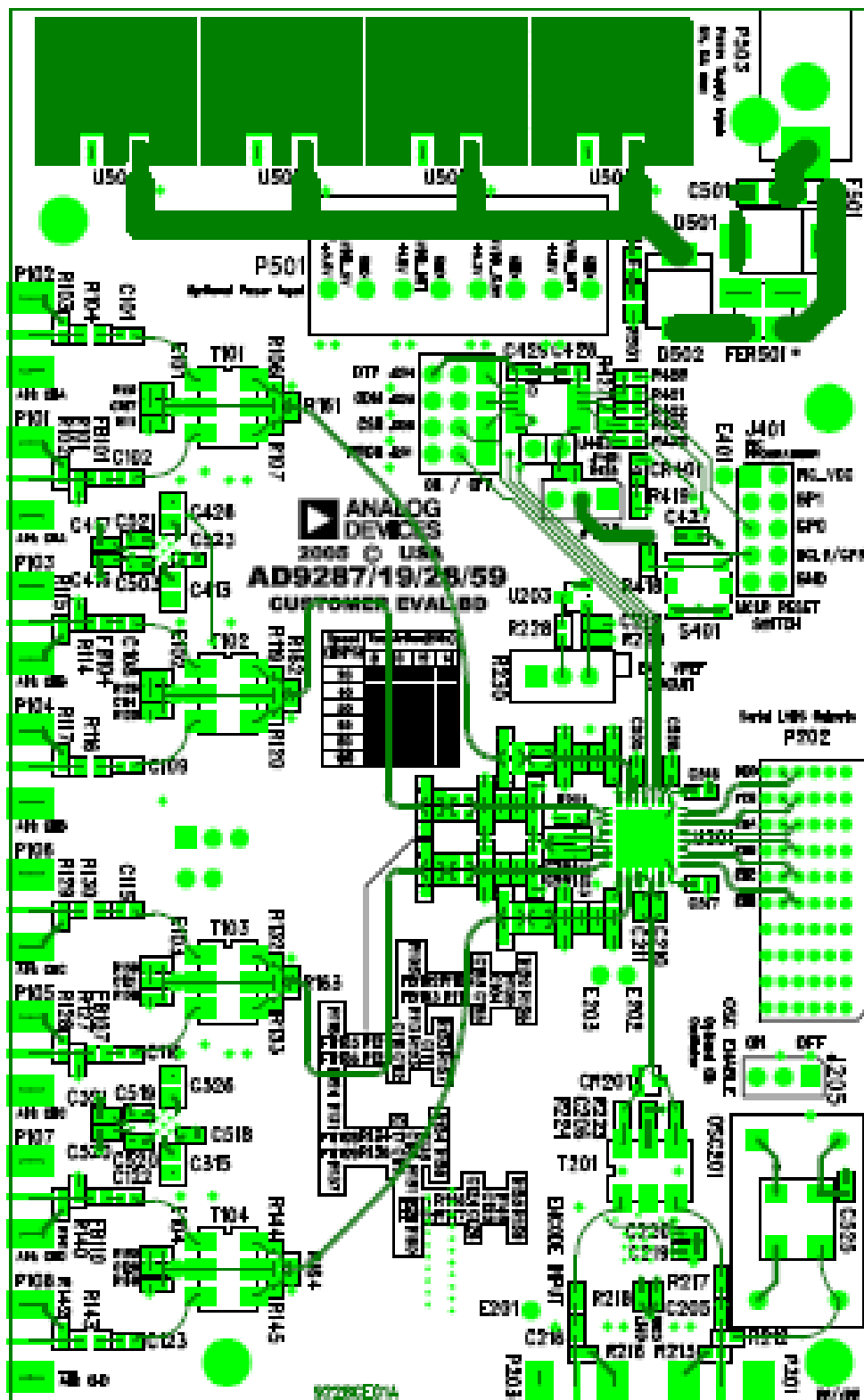
Figure 51. Evaluation Board Layout, Primary Side
