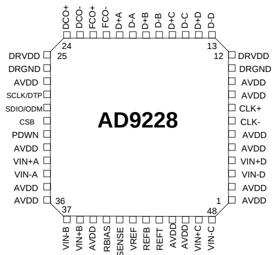
Figure 3. 48LFCSP 7x7 Top View
