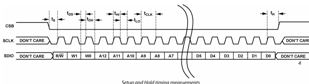
Figure 4645. Serial Timing Details
