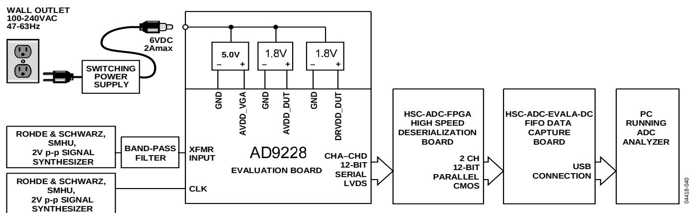
Figure 4846. Evaluation Board Connection
