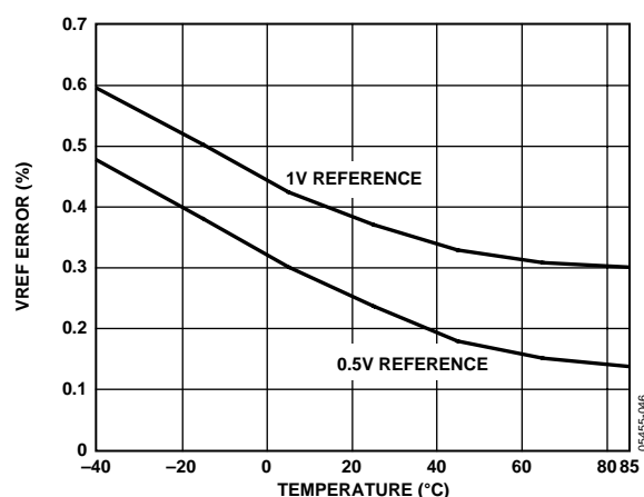
Figure 41. Typical VREF Drift
