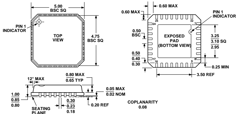
Figure 57. 32-Lead Lead Frame Chip Scale Package [LFCSP_VQ] 5 mm × 5 mm Body, Very Thin Quad (CP-32-2) Dimensions shown in millimeters
