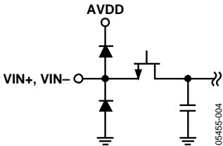
Figure 4. Equivalent Analog Input Circuit
