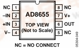
Figure 3. AD8655 8-Lead SOIC (R-8)
