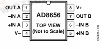
Figure 4. AD8656 8-Lead SOIC (R-8)
