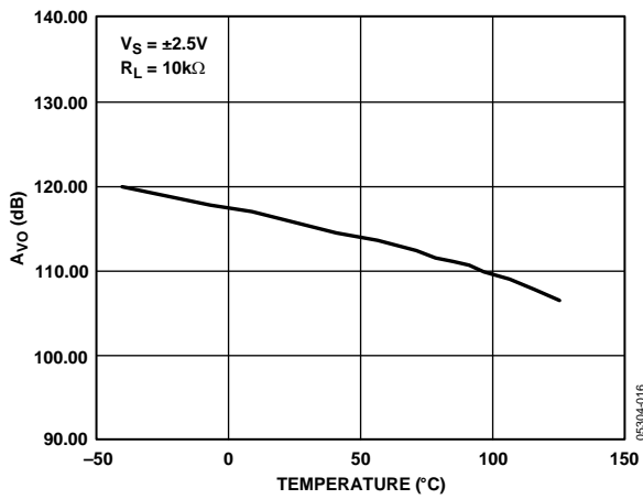
Figure 24. Large Signal Open-Loop Gain vs. Temperature
