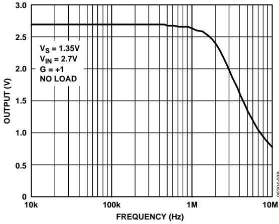
Figure 53. Maximum Output Swing vs. Frequency
