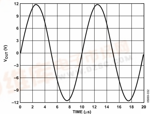
Figure 3. Output Swing, V_S = \pm 12\text{ V} , R_L = 100\ \Omega
