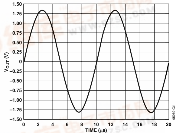
Figure 2. Output Swing, V_S = \pm 1.5\text{ V} , R_L = 25\ \Omega
