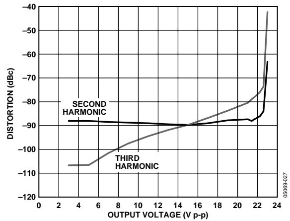
Figure 21. Distortion vs. Output Voltage @ 100 kHz, ( V_S = \pm 12\text{ V} , G = +5 , R_L = 50\ \Omega )
