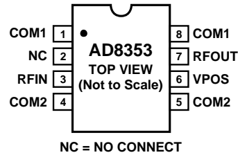
Figure 2. Pin Configuration
