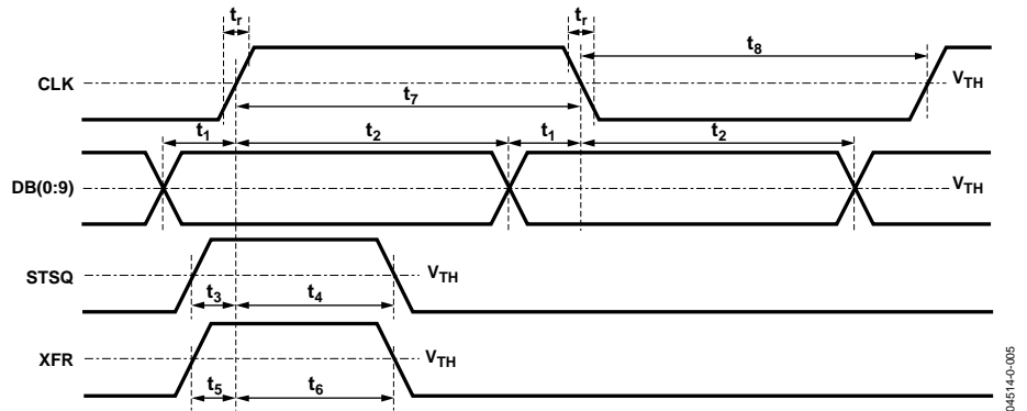
Figure 5. Input Timing
