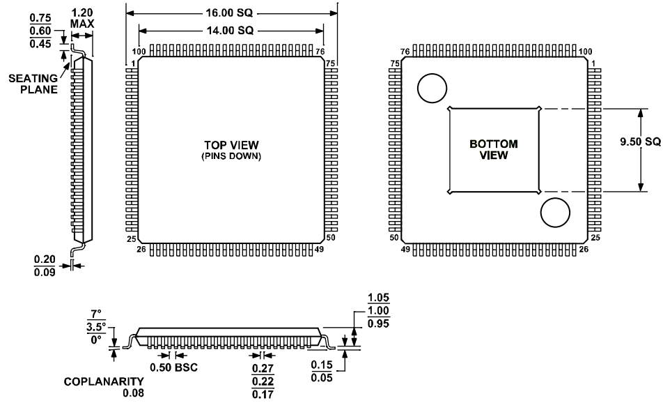
Figure 25. 100-Lead, Thermally Enhanced Thin Quad Flat Package (with Exposed Heat Sink) [TQFP_EP]
