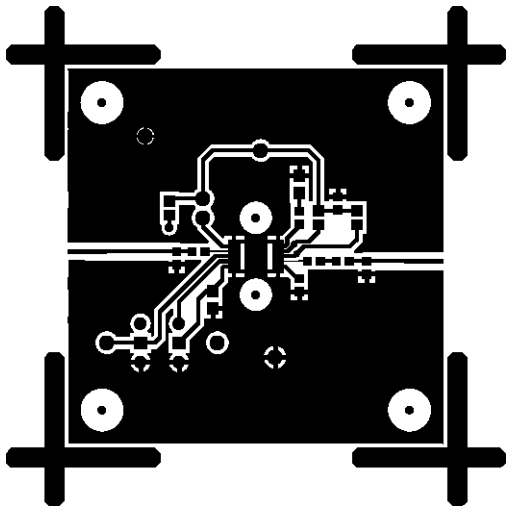
Figure 43. Layout of Component Side
