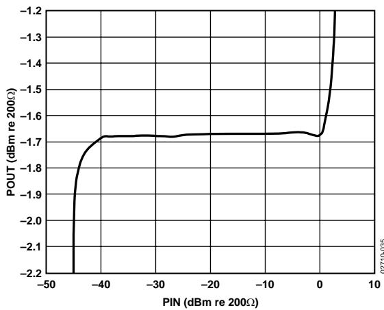
Figure 35. Leveling Accuracy of the AGC Function
