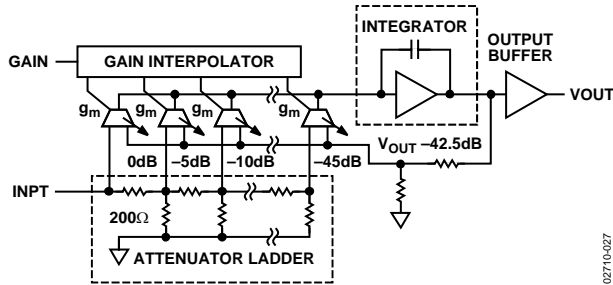
Figure 27. Simplified Architecture
