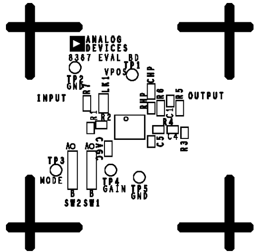
Figure 44. Silkscreen of Component Side
