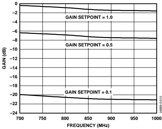
Figure 10. Gain vs. Frequency at Different Gain Setpoints (700 MHz to 1000 MHz), Phase Setpoint = 0°
