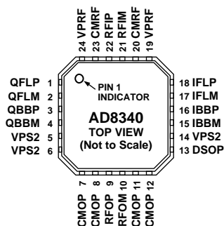
Figure 2. 24-Lead Lead Frame Chip Scale Package (LFCS)
