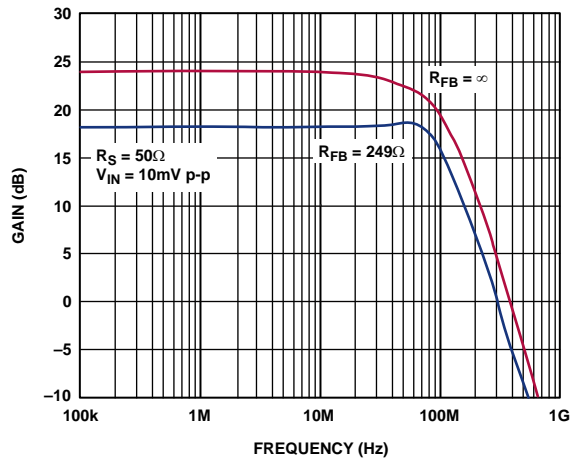
Figure 12. Frequency Response for a Terminated and Unterminated 50\ \Omega Source (See Figure 49)
