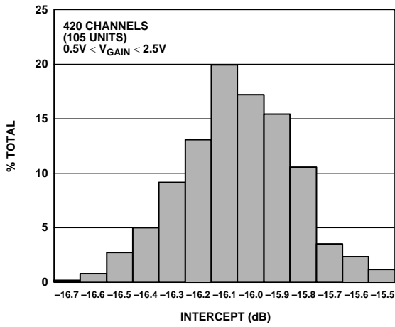
Figure 9. Intercept Histogram
