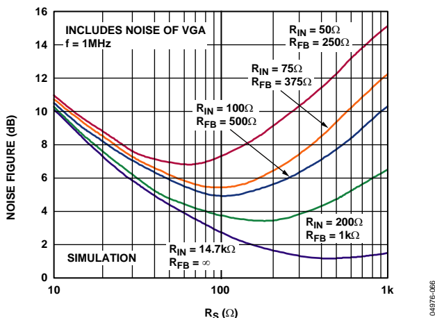
Figure 56. Simulated Noise Figure vs. R_S for Various Fixed Values of R_{IN} , Actively Matched
