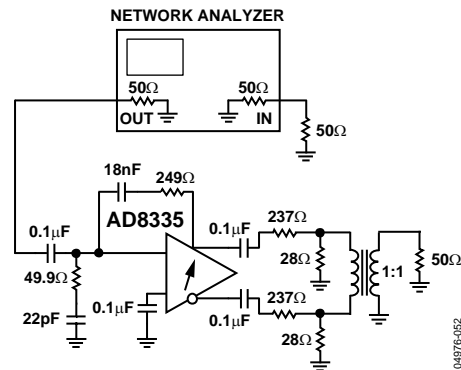
Figure 52. Test Circuit Used for S11 Measurements
