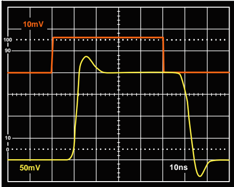
Figure 39. Large Signal Pulse Response, LO Gain (See Figure 51)
