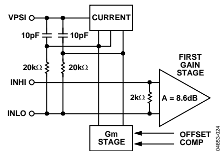
Figure 24. Input Interface
