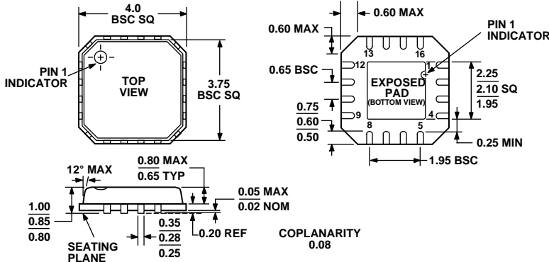
COMPLIANT TO JEDEC STANDARDS MO-220-VGGC Figure 48. 16-Lead Lead Frame Chip Scale Package [LFCSP] (CP-16) Dimensions shown in millimeters
