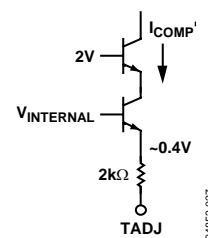
Figure 27. TADJ Interface
