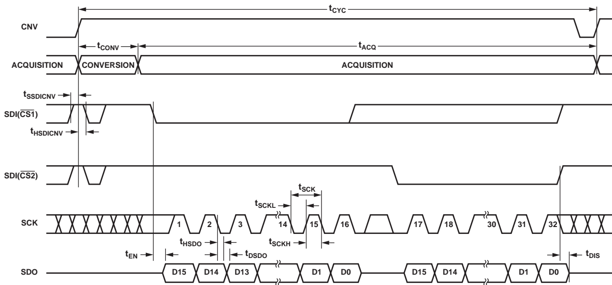
Figure 23. \overline{CS} Mode 4-Wire, No BUSY Indicator Serial Interface Timing
