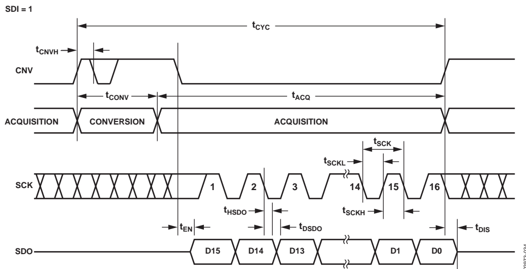
Figure 19. \overline{CS} Mode 3-Wire, No BUSY Indicator Serial Interface Timing (SDI High)
