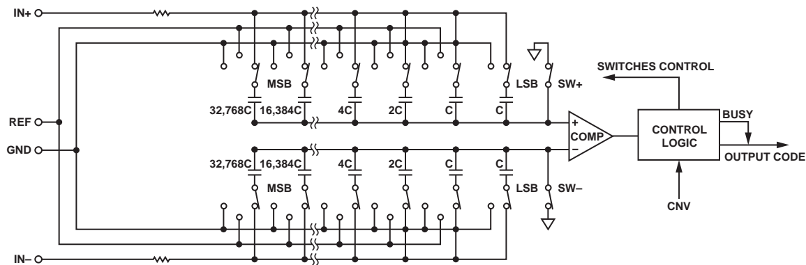
Figure 12. ADC Simplified Schematic
