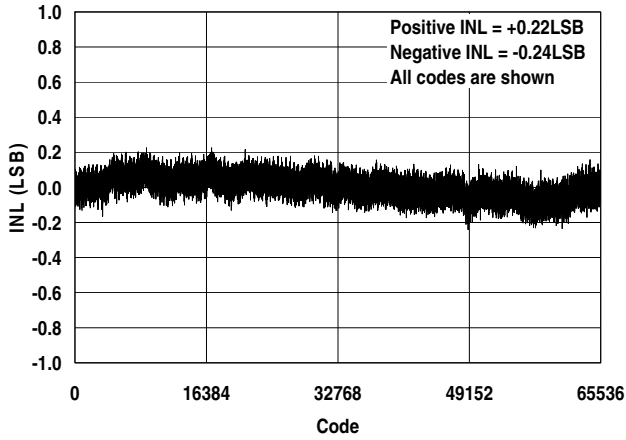
Figure 7. Integral Nonlinearity vs. Code
