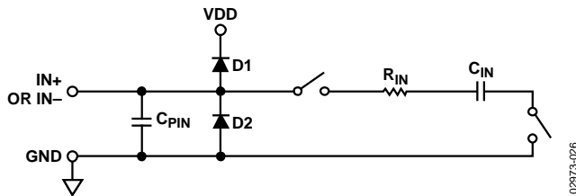
Figure 16. Equivalent Analog Input Circuit
