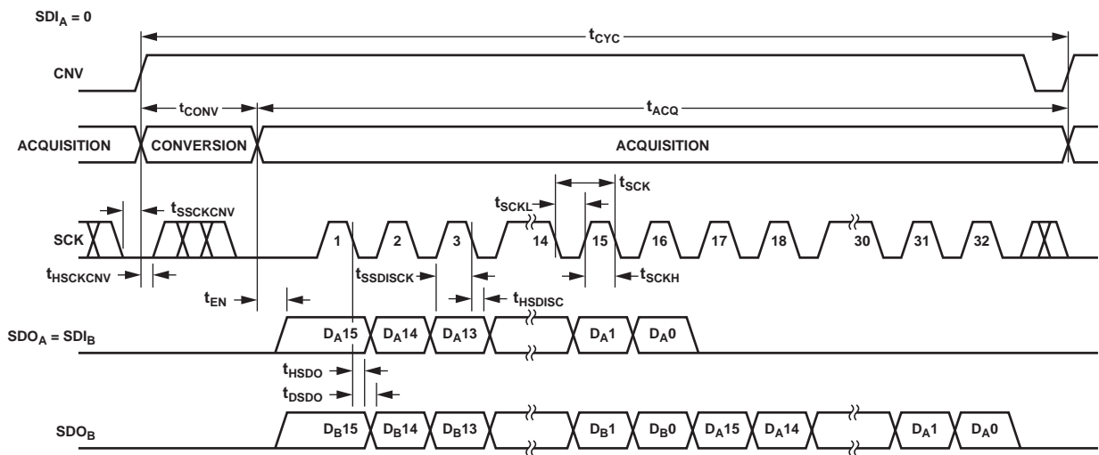
Figure 27. Chain Mode, No BUSY Indicator Serial Interface Timing
