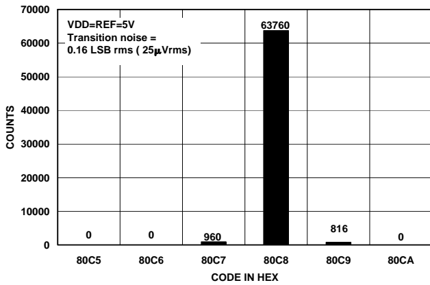
Figure 8. Histogram of a DC Input at the Code Center
