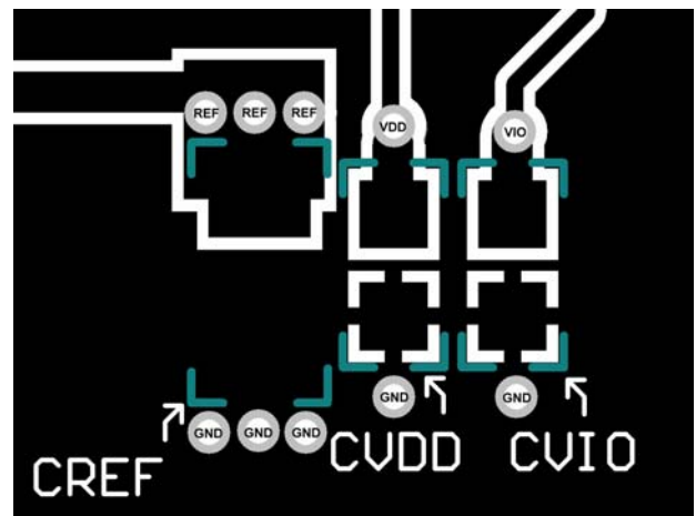
Figure 31. Example of Layout of the AD7693 (Bottom Layer)
