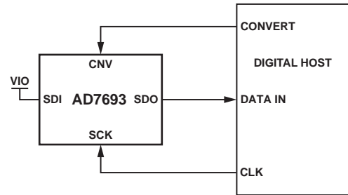
Figure 18. \overline{CS} Mode 3-Wire, No BUSY Indicator Connection Diagram (SDI High)
