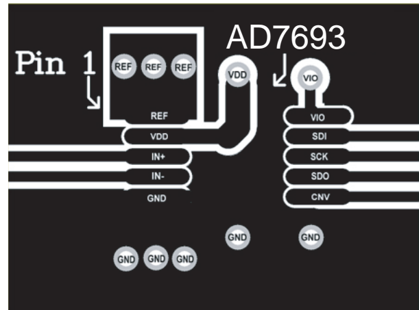
Figure 30. Example of Layout of the AD7693 (Top Layer)
