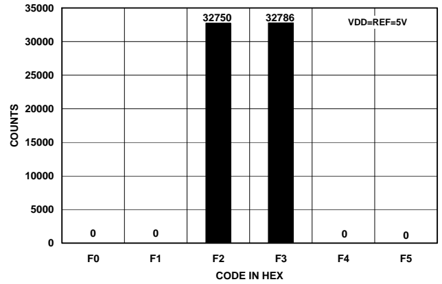
Figure 11. Histogram of a DC Input at the Code Transition
