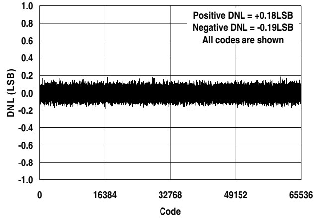
Figure 10. Differential Nonlinearity vs. Code
