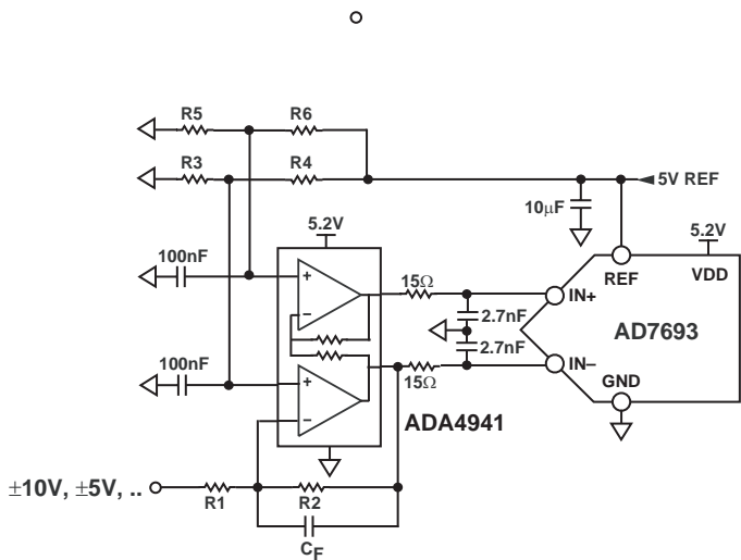
Figure 17. Single-Ended-to-Differential Driver Circuit
