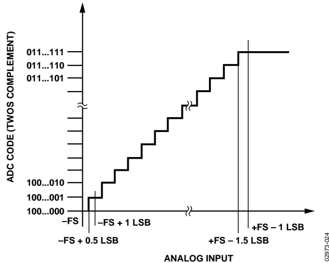
Figure 13. ADC Ideal Transfer Function
