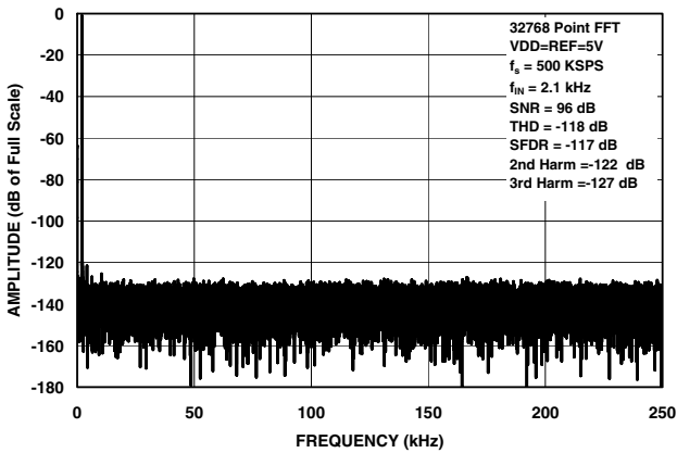
Figure 9. FFT Plot
