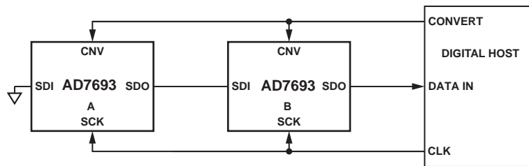
Figure 26. Chain Mode, No BUSY Indicator Connection Diagram
