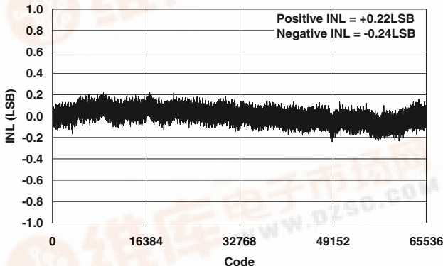
Figure 1. Integral Nonlinearity vs. Code
