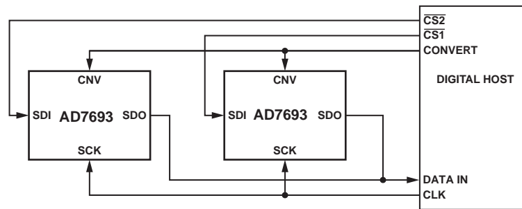
Figure 22. \overline{CS} Mode 4-Wire, No BUSY Indicator Connection Diagram
