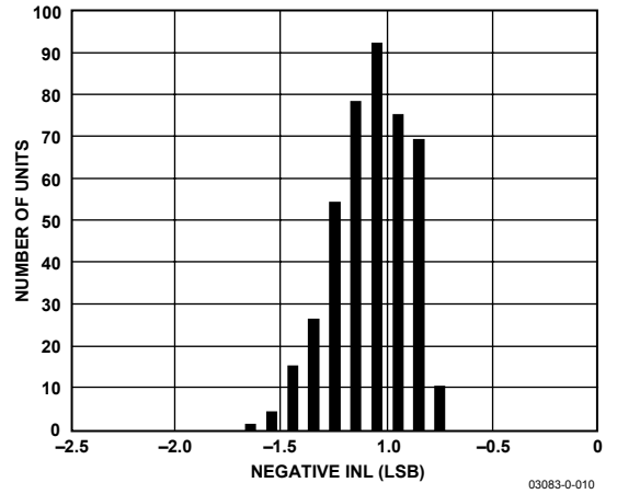
Figure 10. Typical Negative INL Distribution (424 Units)
