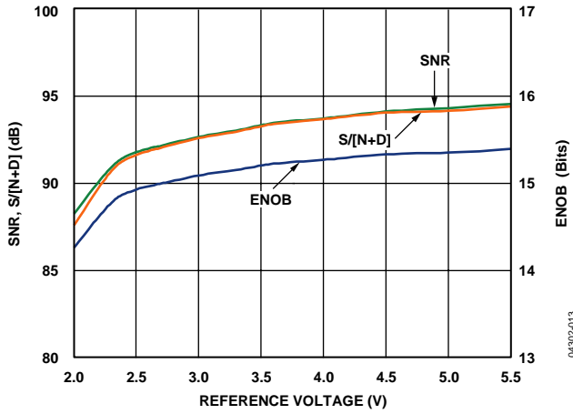
Figure 13. SNR, S/(N+D) , and ENOB vs. Reference Voltage
