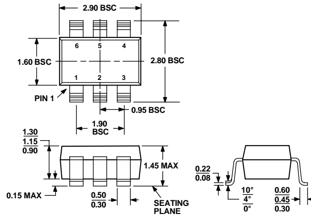
Figure 23. 6-Lead Small Outline Transistor Package [SOT-23] (RJ-6) Dimensions shown in millimeters
