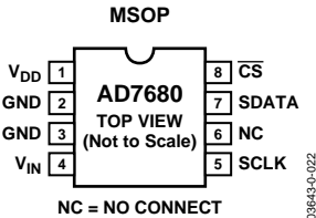
Figure 4. MSOP Pin Configuration
