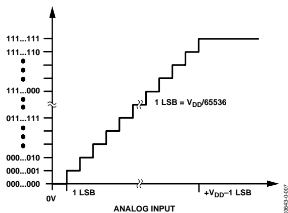
Figure 14. AD7680 Transfer Characteristic
