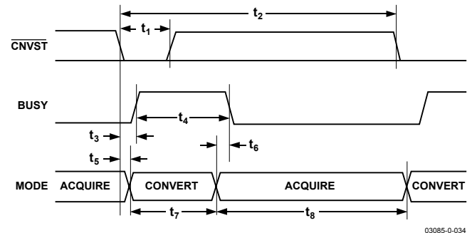
Figure 32. Basic Conversion Timing
